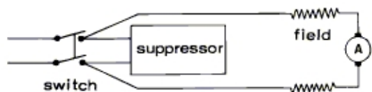
WIRING DIAGRAM
